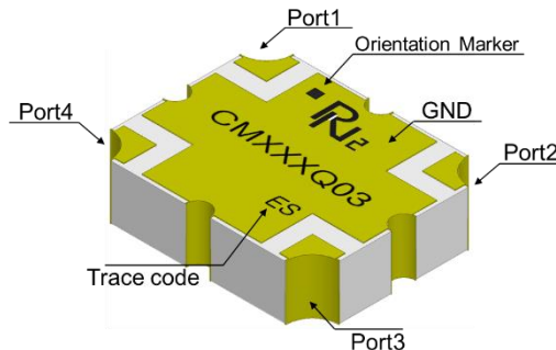
Figure 1. CMX35Q03 (Top View)
