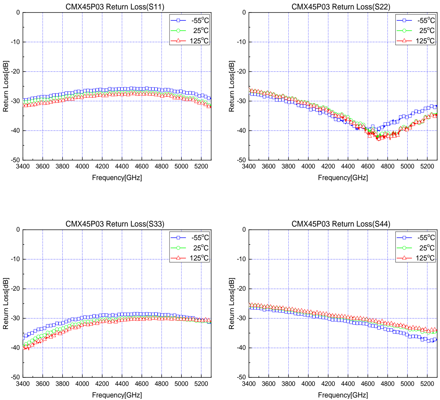
Figure 3. Test Plots of Return Loss (at -55 °C, 25 °C, and 125 °C)
