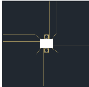
Figure 11. Placing the CMX45P03 on the 6Points of the PCB Surface
