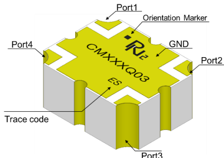
Figure 1. CMX50Q03 (Top View)
