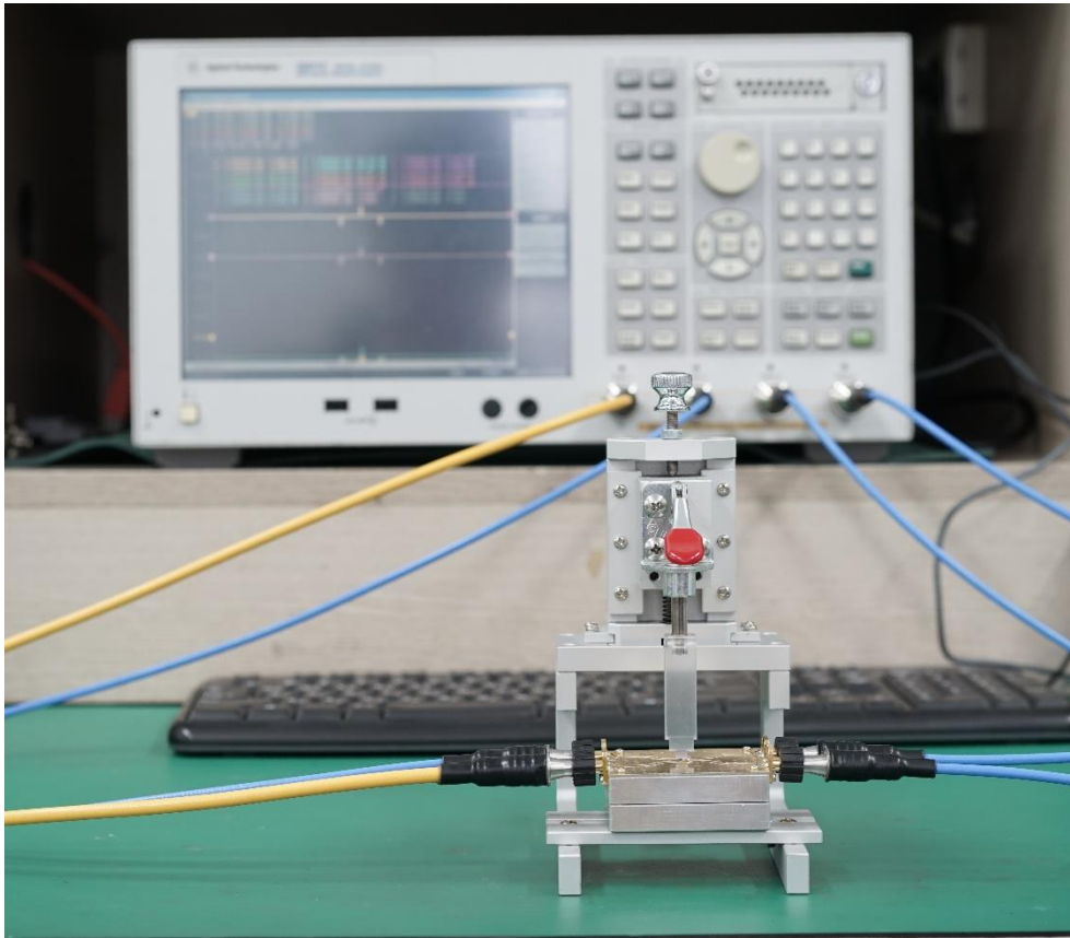
Figure 5. Test Setting to Measure the CMX50Q03 S-parameters
