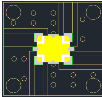
Figure 11. Placing the CMX50Q03 on the 9 Points of the PCB Surface
