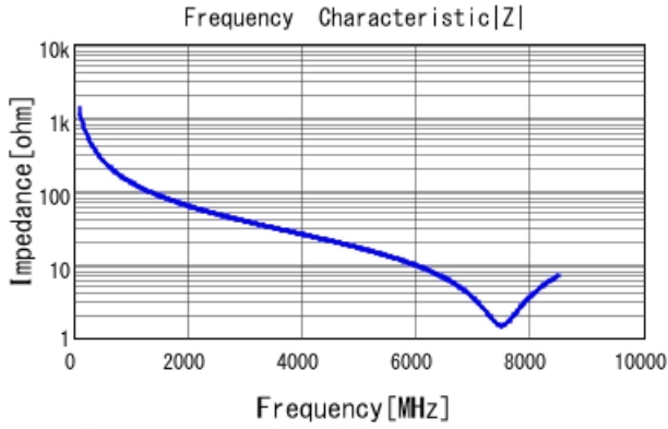
GRM1555C1H1R2BA01 |Z| DCOV, 25degC
