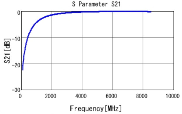
GRM1555C1H1R2BA01 S21 DCOV, 25degC
