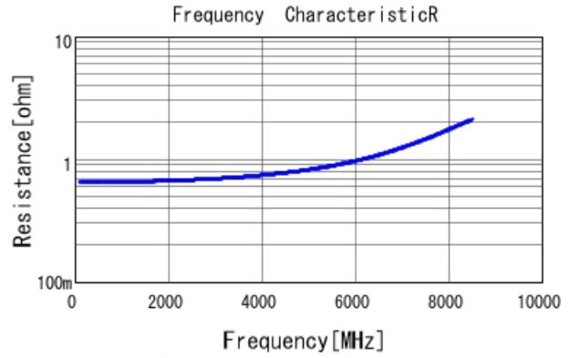
GRM1555C1H1R2BA01 R DCOV, 25degC
