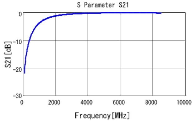
GRM1555C1H1R3CA01 S21 DCOV, 25degC
