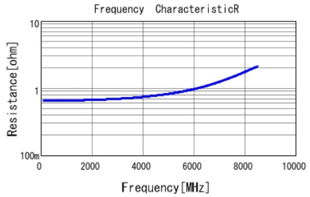
GRM1555C1H1R3CA01 R DCOV, 25degC
