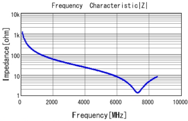
GRM1555C1H1R3CA01 |Z| DCOV, 25degC
