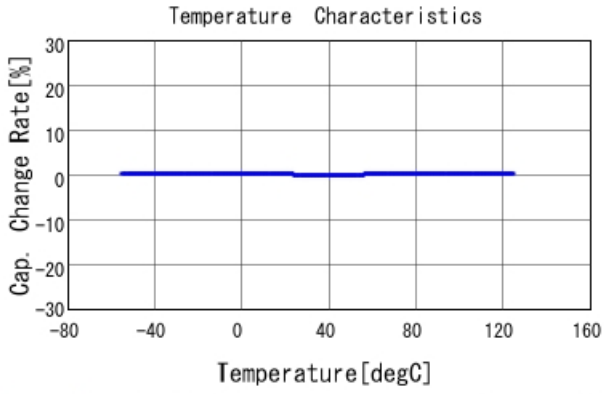
GRM1555C1H1R3CA01 C-Temp. capchange, DCOV, AC1Vrms
