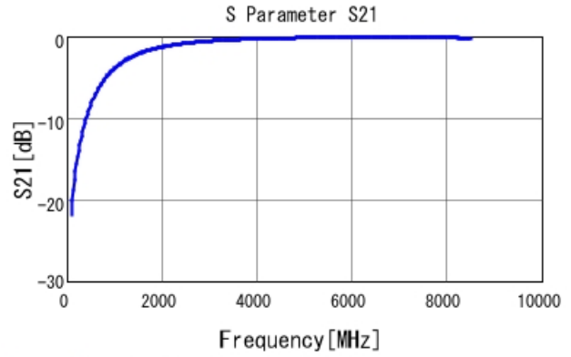
GRM1555C1H1R3WA01 S21 DCOV, 25degC
