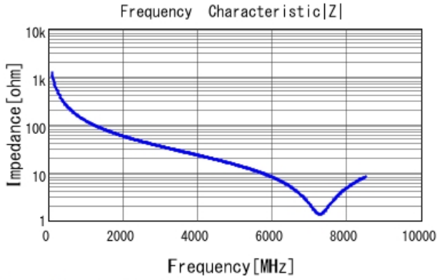
GRM1555C1H1R3WA01 |Z| DCOV, 25degC
