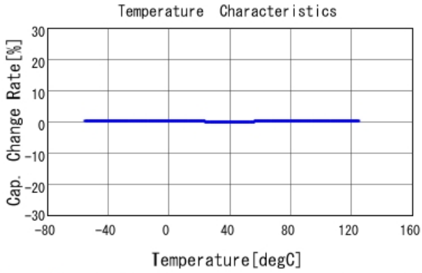
GRM1555C1H1R3WA01 C-Temp. capchange, DCOV, AC1Vrms
