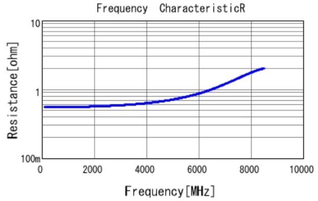
GRM1555C1H1R5CA01 R DCOV, 25degC
