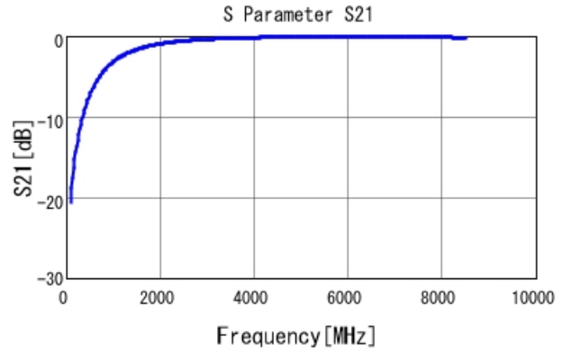
GRM1555C1H1R5CA01 S21 DCOV, 25degC
