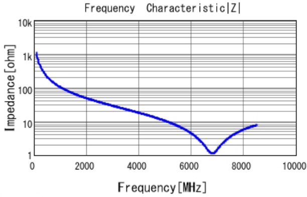
GRM1555C1H1R5CA01 |Z| DCOV, 25degC
