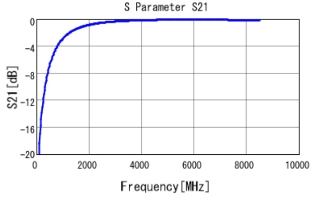
GRM1555C1H1R6CA01 S21 DCOV, 25degC
