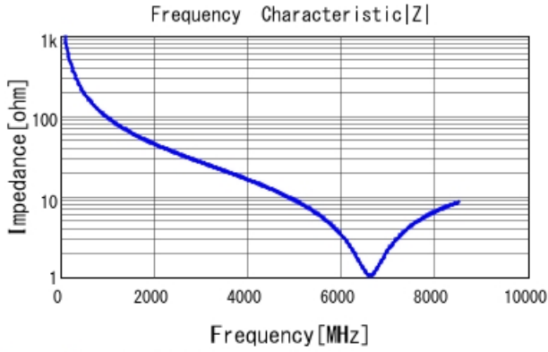
GRM1555C1H1R6CA01 |Z| DCOV, 25degC
