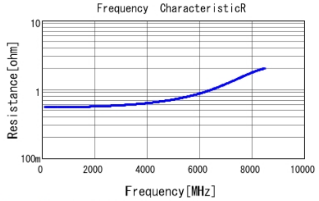
GRM1555C1H1R6CA01 R DCOV, 25degC
