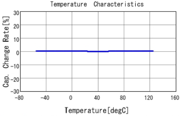
GRM1555C1H1R6WA01 C-Temp. capchange, DCOV, AC1Vrms
