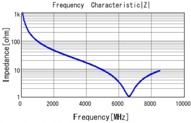
GRM1555C1H1R6WA01 |Z| DCOV, 25degC
