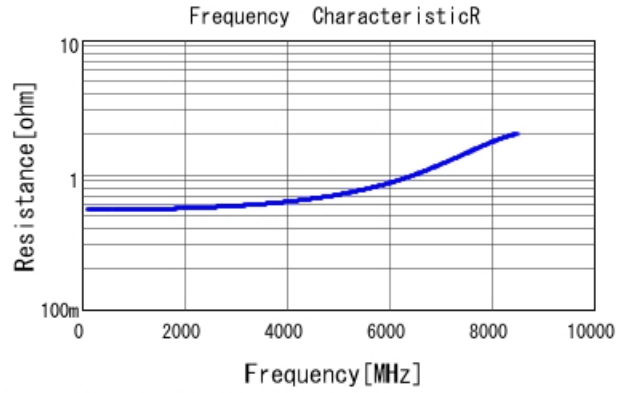
GRM1555C1H1R6WA01 R DCOV, 25degC
