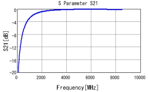
GRM1555C1H1R6WA01 S21 DCOV, 25degC
