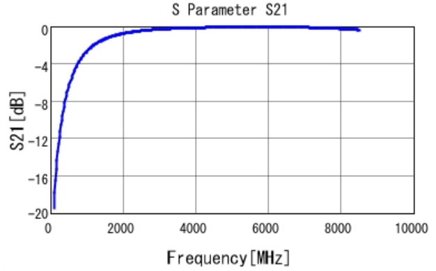
GRM1555C1H1R7BA01 S21 DCOV, 25degC
