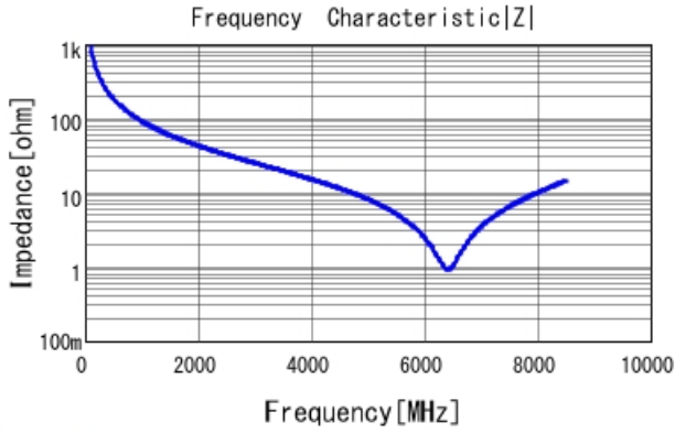
GRM1555C1H1R7BA01 |Z| DCOV, 25degC
