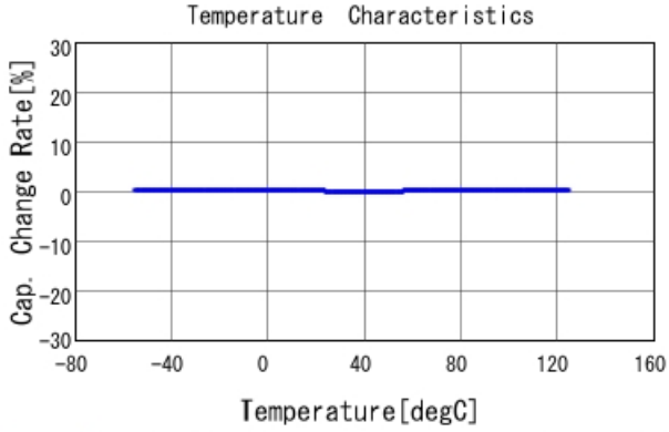
GRM1555C1H1R7BA01 C-Temp. capchange, DCOV, AC1Vrms
