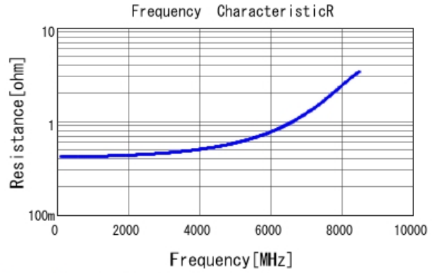
GRM1555C1H1R7BA01 R DCOV, 25degC
