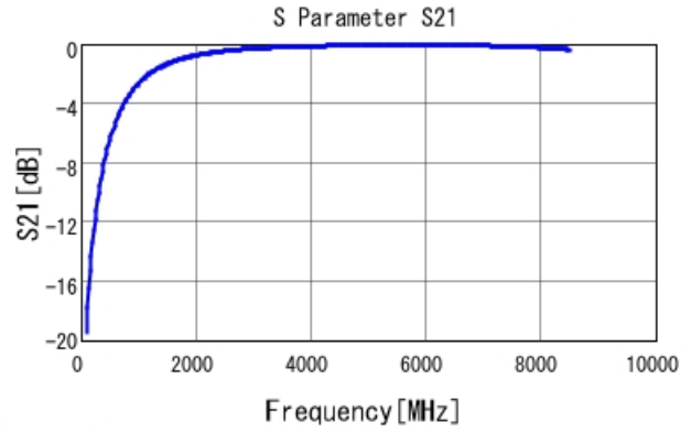
GRM1555C1H1R7CA01 S21 DCOV, 25degC
