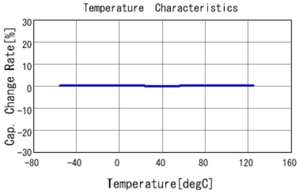
GRM1555C1H1R7CA01 C-Temp. capchange, DCOV, AC1Vrms
