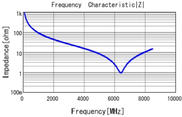
GRM1555C1H1R7CA01 |Z| DCOV, 25degC
