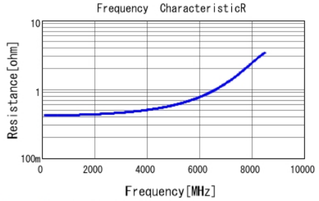
GRM1555C1H1R7CA01 R DCOV, 25degC
