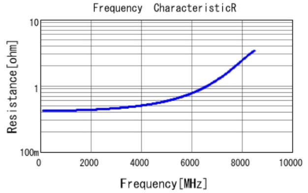
GRM1555C1H1R7WA01 R DCOV, 25degC
