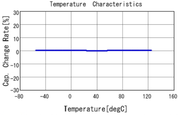
GRM1555C1H1R7WA01 C-Temp. capchange, DCOV, AC1Vrms
