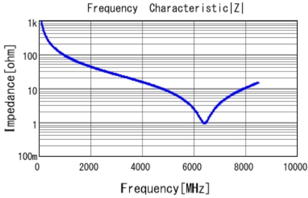
GRM1555C1H1R7WA01 |Z| DCOV, 25degC
