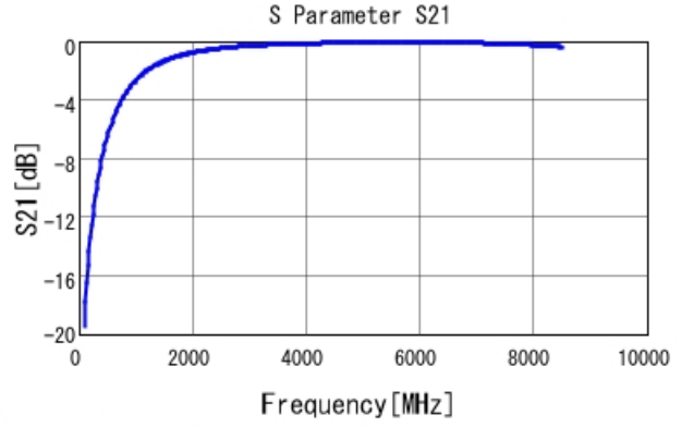
GRM1555C1H1R7WA01 S21 DCOV, 25degC
