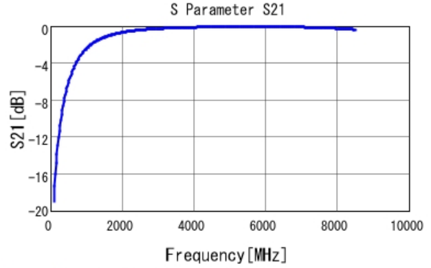
GRM1555C1H1R8CA01 S21 DCOV, 25degC
