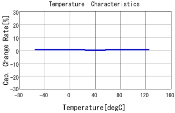
GRM1555C1H1R8CA01 C-Temp. capchange, DCOV, AC1Vrms
