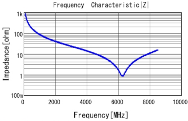
GRM1555C1H1R8CA01 |Z| DCOV, 25degC
