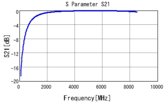
GRM1555C1H1R9BA01 S21 DCOV, 25degC
