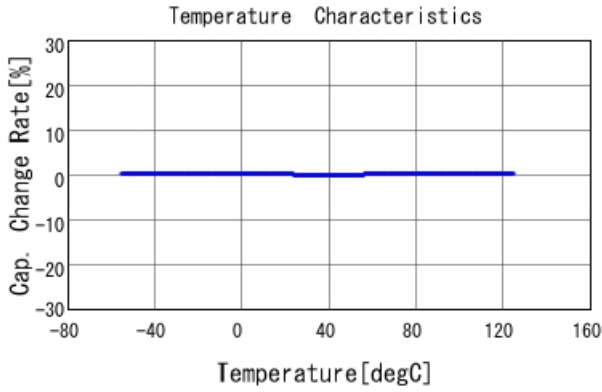
GRM1555C1H1R9BA01 C-Temp. capchange, DCOV, AC1Vrms
