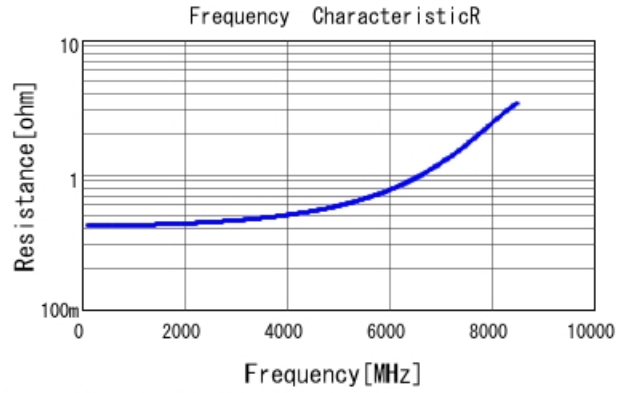
GRM1555C1H1R9BA01 R DCOV, 25degC
