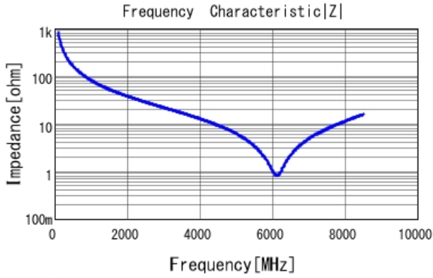
GRM1555C1H1R9BA01 |Z| DCOV, 25degC
