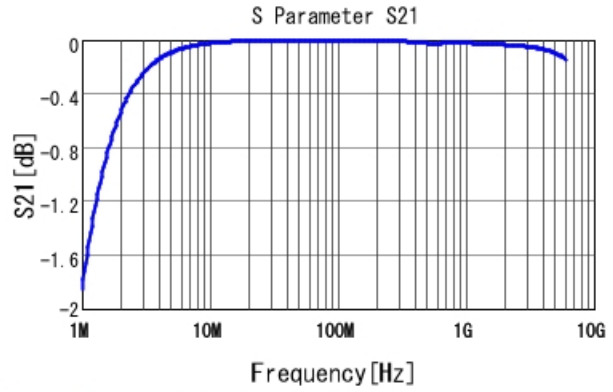
GRM1555C1H222GA01 S21 DCOV, 25degC
