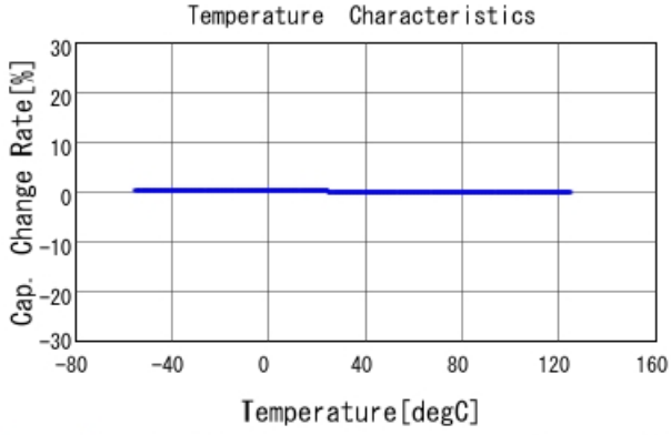
GRM1555C1H222JA01 C-Temp. capchange, DCOV, AC1Vrms
