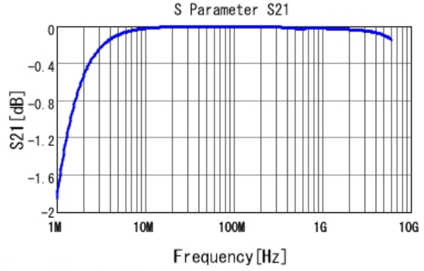
GRM1555C1H222JA01 S21 DCOV, 25degC
