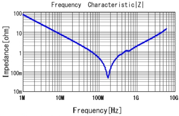
GRM1555C1H222JA01 |Z| DCOV, 25degC
