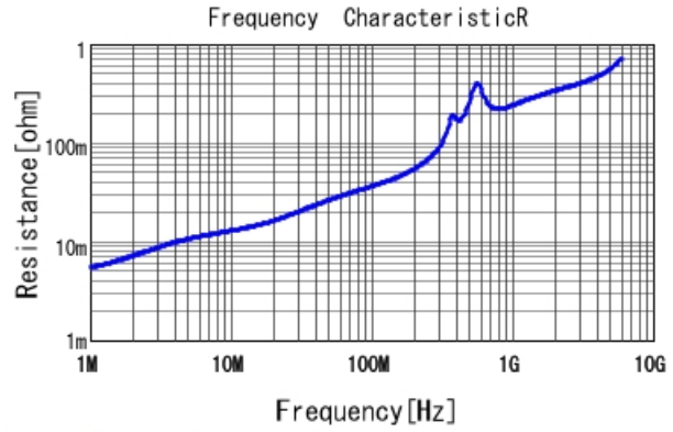
GRM1555C1H222JA01 R DCOV, 25degC
