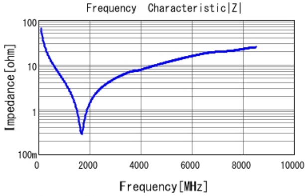
GRM1555C1H240JA01 |Z| DCOV, 25degC
