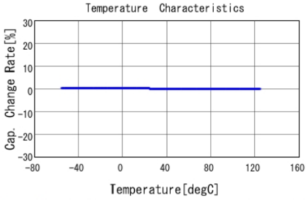
GRM1555C1H240JA01 C-Temp. capchange, DCOV, AC1Vrms
