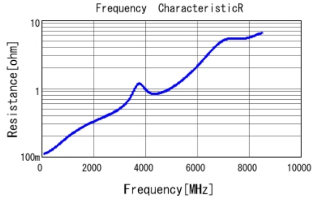
GRM1555C1H240JA01 R DCOV, 25degC
