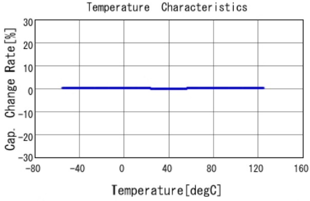
GRM1555C1H2R1BA01 C-Temp. capchange, DCOV, AC1Vrms
