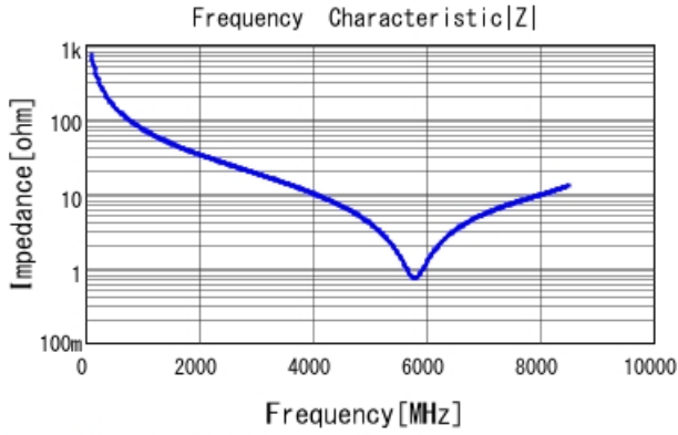
GRM1555C1H2R1BA01 |Z| DCOV, 25degC
