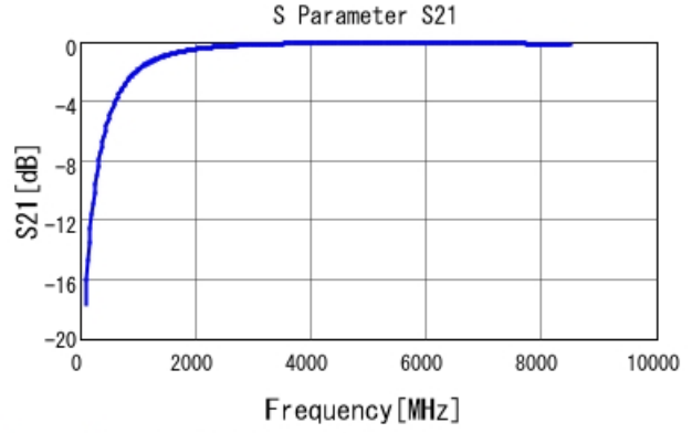
GRM1555C1H2R1BA01 S21 DCOV, 25degC
