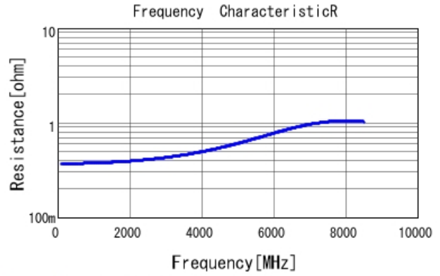
GRM1555C1H2R1BA01 R DCOV, 25degC
