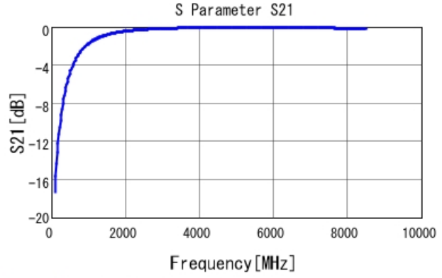
GRM1555C1H2R2BA01 S21 DC0V, 25degC
