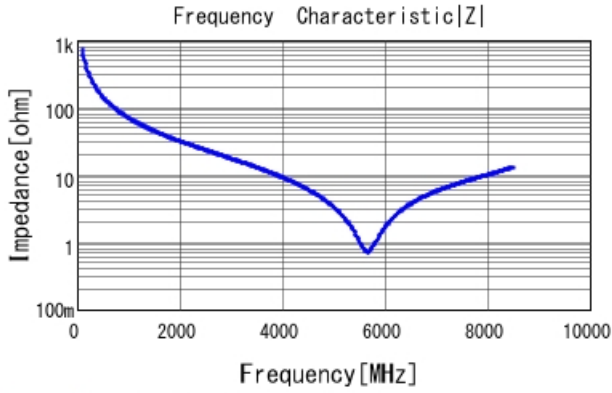
GRM1555C1H2R2BA01 |Z| DCOV, 25degC
