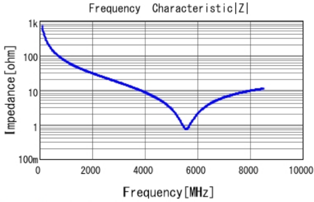
GRM1555C1H2R3WA01 |Z| DCOV, 25degC
