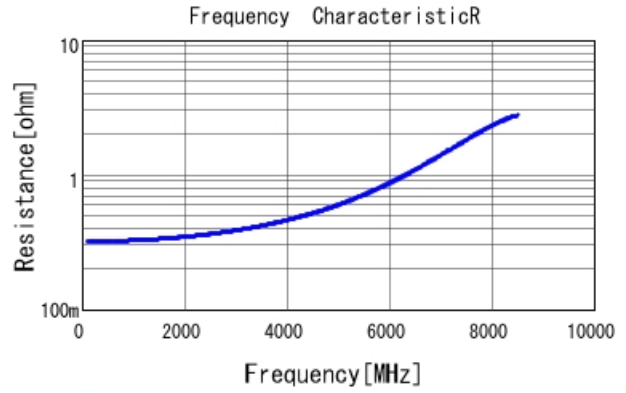
GRM1555C1H2R3WA01 R DCOV, 25degC
