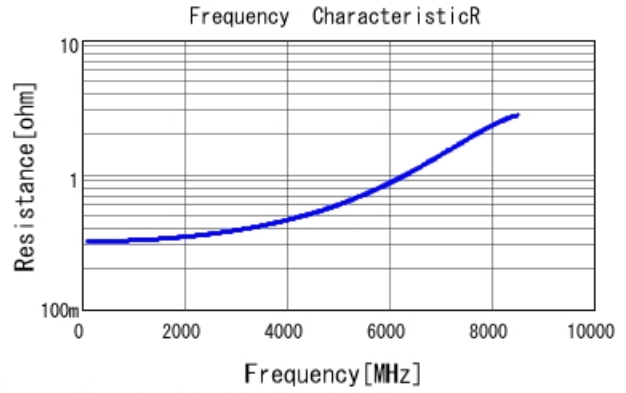
GRM1555C1H2R4BA01 R DCOV, 25degC
