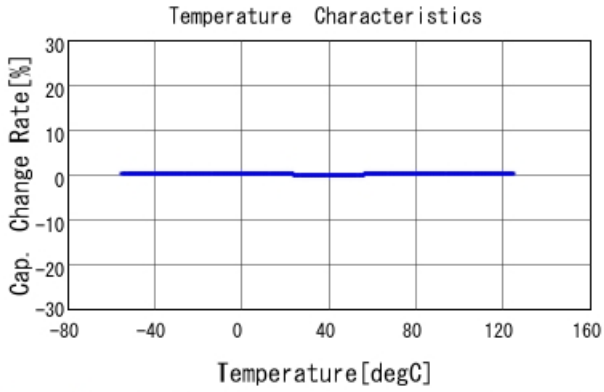
GRM1555C1H2R4BA01 C-Temp. capchange, DC0V, AC1Vrms
