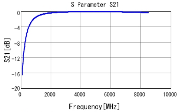
GRM1555C1H2R4BA01 S21 DC0V, 25degC
