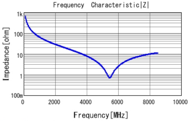
GRM1555C1H2R4BA01 |Z| DCOV, 25degC
