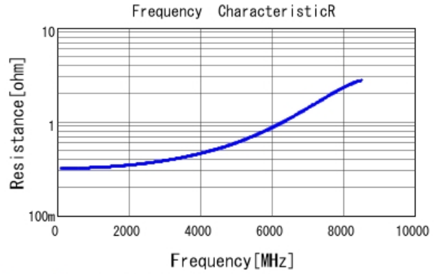
GRM1555C1H2R4WA01 R DCOV, 25degC
