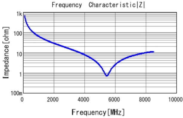
GRM1555C1H2R4WA01 |Z| DCOV, 25degC
