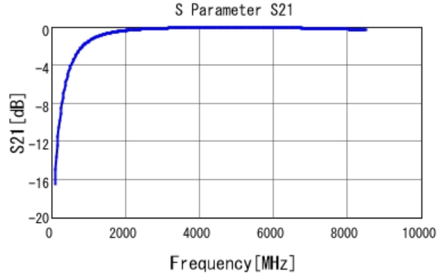
GRM1555C1H2R4WA01 S21 DCOV, 25degC
