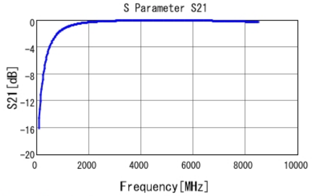
GRM1555C1H2R5BA01 S21 DC0V, 25degC
