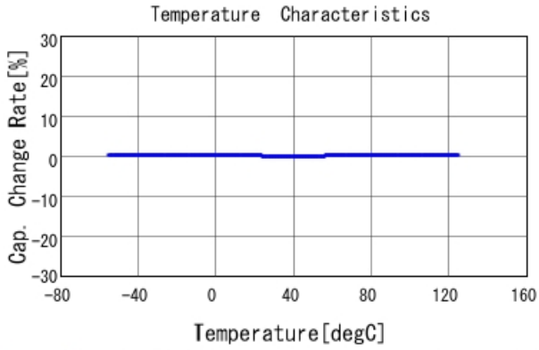
GRM1555C1H2R5BA01 C-Temp. capchange, DC0V, AC1Vrms
