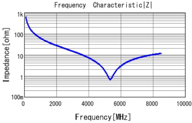
GRM1555C1H2R5BA01 |Z| DCOV, 25degC
