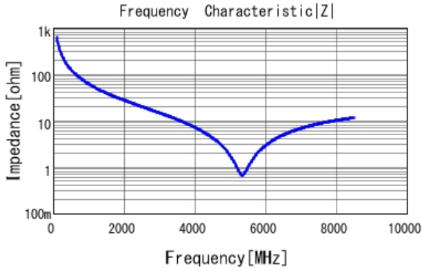
GRM1555C1H2R5WA01 |Z| DCOV, 25degC
