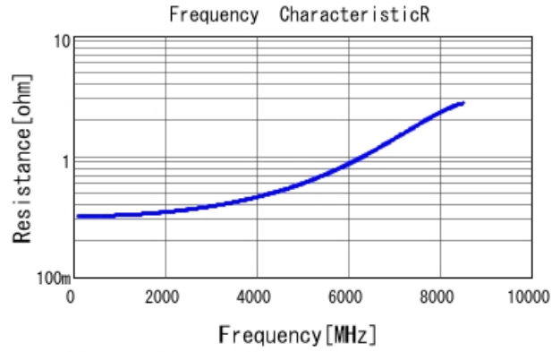
GRM1555C1H2R5WA01 R DCOV, 25degC
