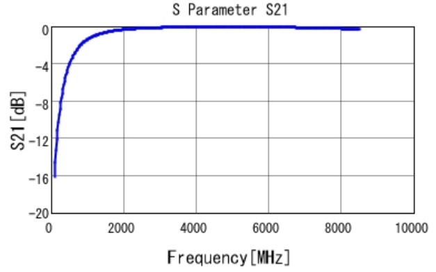
GRM1555C1H2R5WA01 S21 DC0V, 25degC
