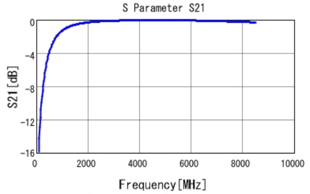
GRM1555C1H2R6WA01 S21 DCOV, 25degC
