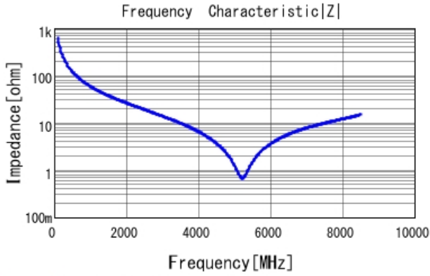
GRM1555C1H2R6WA01 |Z| DCOV, 25degC
