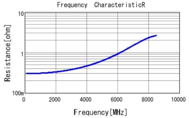
GRM1555C1H2R6WA01 R DCOV, 25degC
