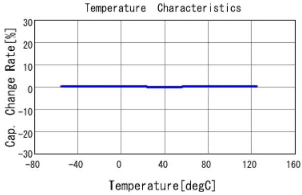
GRM1555C1H2R6WA01 C-Temp. capchange, DCOV, AC1Vrms
