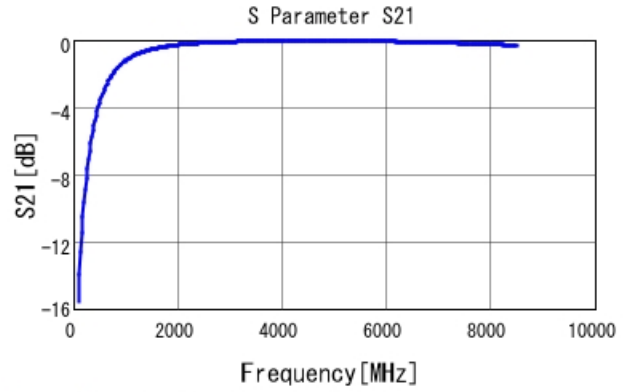
GRM1555C1H2R7WA01 S21 DCOV, 25degC
