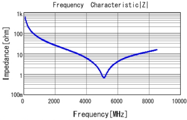
GRM1555C1H2R7WA01 |Z| DCOV, 25degC
