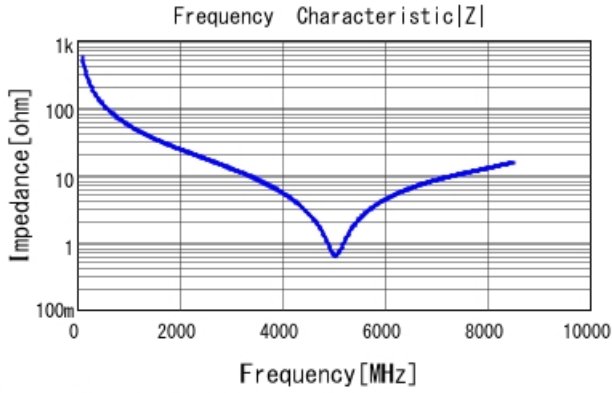
GRM1555C1H2R8BA01 |Z| DCOV, 25degC
