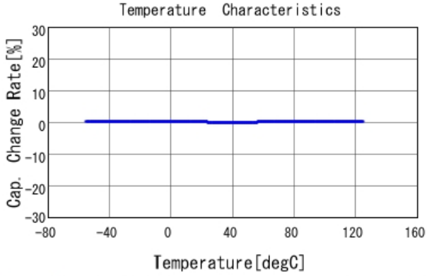
GRM1555C1H2R8BA01 C-Temp. capchange, DCOV, AC1Vrms
