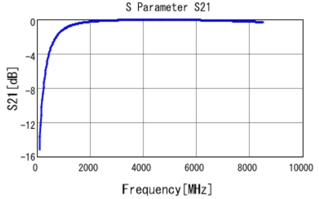
GRM1555C1H2R8BA01 S21 DCOV, 25degC
