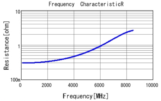
GRM1555C1H2R8BA01 R DCOV, 25degC
