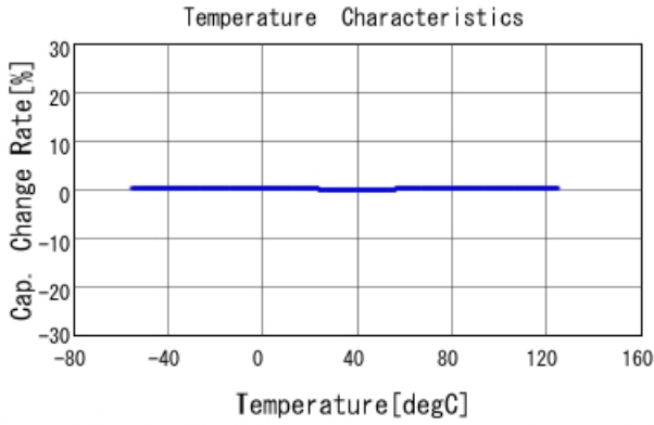
GRM1555C1H2R9BA01 C-Temp. capchange, DCOV, AC1Vrms
