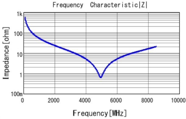
GRM1555C1H2R9BA01 |Z| DCOV, 25degC
