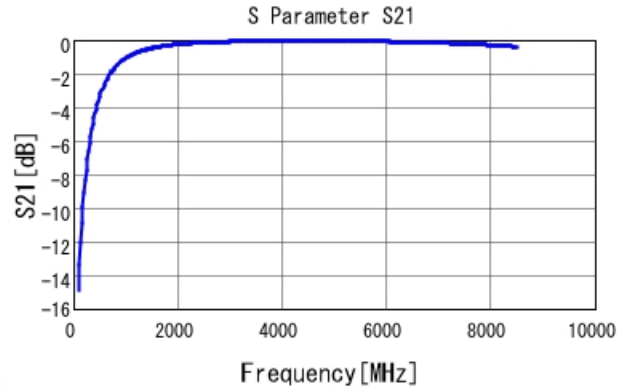
GRM1555C1H2R9BA01 S21 DCOV, 25degC
