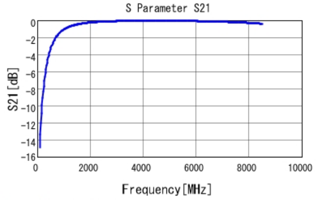
GRM1555C1H2R9CA01 S21 DCOV, 25degC
