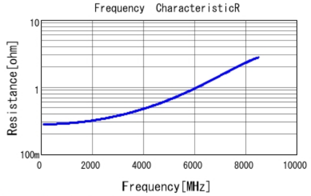
GRM1555C1H2R9CA01 R DCOV, 25degC
