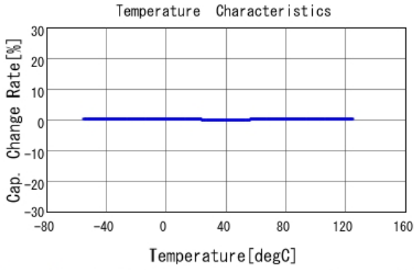
GRM1555C1H2R9CA01 C-Temp. capchange, DCOV, AC1Vrms
