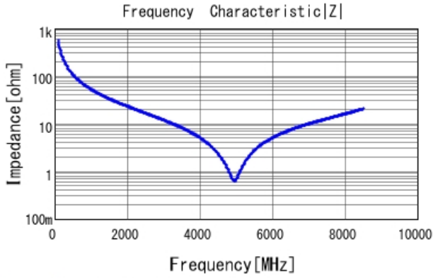
GRM1555C1H2R9CA01 |Z| DCOV, 25degC
