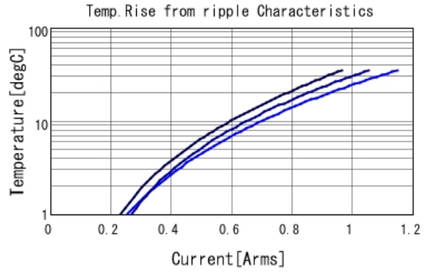
GRM1555C1H390GA01 Temp. rise — 500MHz — 700I
