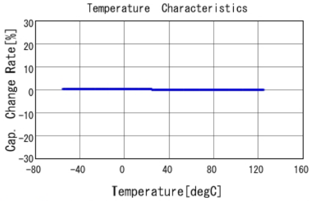
GRM1555C1H390GA01 C-Temp. capchange, DCOV, AC1Vrms
