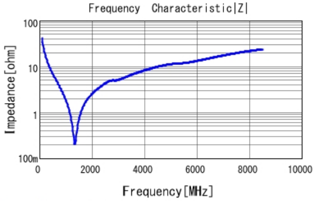
GRM1555C1H390GA01 |Z| DCOV, 25degC
