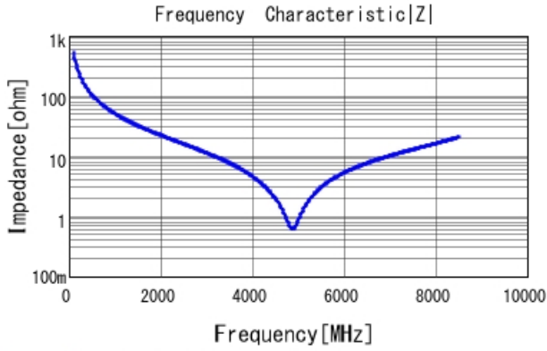
GRM1555C1H3R0WA01 |Z| DCOV, 25degC
