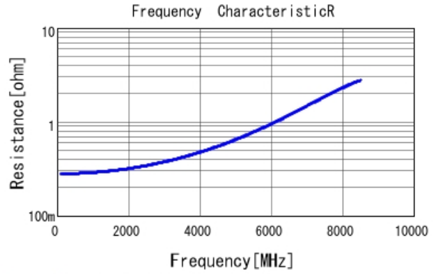
GRM1555C1H3R0WA01 R DCOV, 25degC
