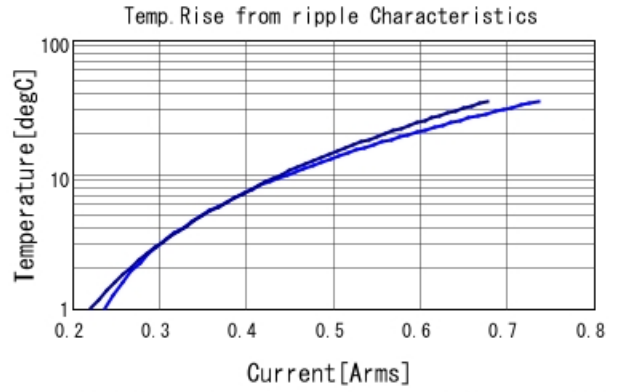
GRM1555C1H3R0WA01 Temp. rise — 2GHz — 3GHz
