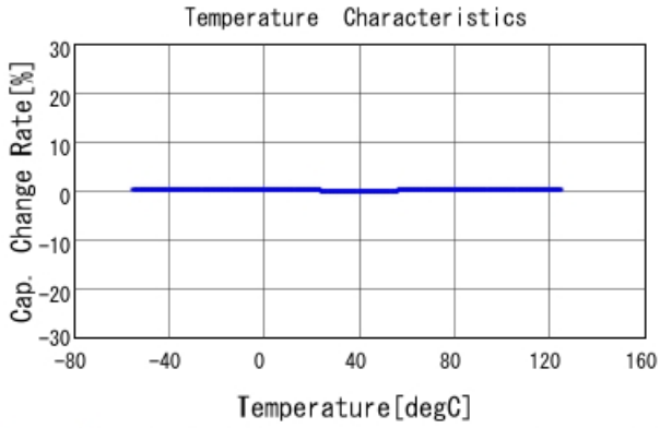
GRM1555C1H3R0WA01 C-Temp. capchange, DCOV, AC1Vrms
