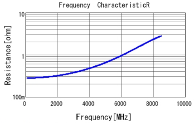
GRM1555C1H3R1BA01 R DCOV, 25degC
