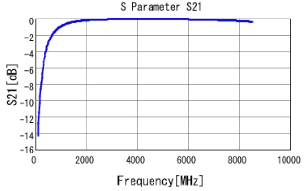
GRM1555C1H3R1BA01 S21 DCOV, 25degC
