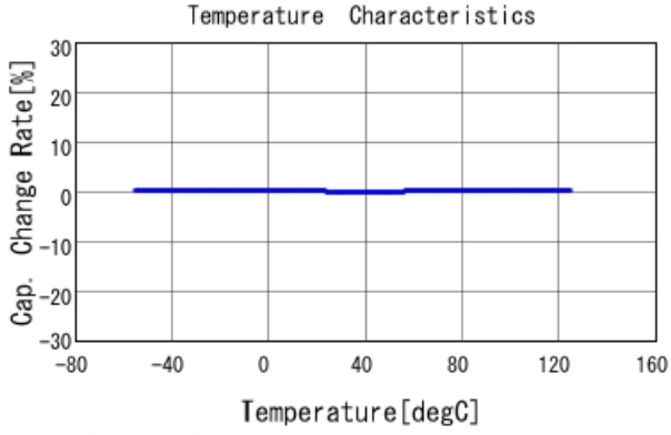
GRM1555C1H3R1BA01 C-Temp. capchange, DCOV, AC1Vrms
