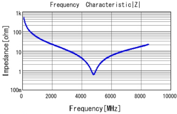
GRM1555C1H3R1BA01 |Z| DCOV, 25degC
