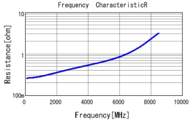
GRM1555C1H3R2CA01 R DCOV, 25degC
