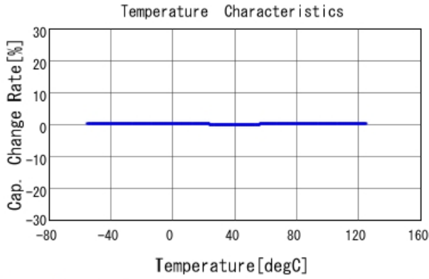
GRM1555C1H3R2CA01 C-Temp. capchange, DC0V, AC1Vrms
