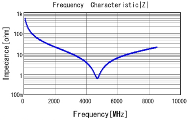
GRM1555C1H3R2CA01 |Z| DCOV, 25degC
