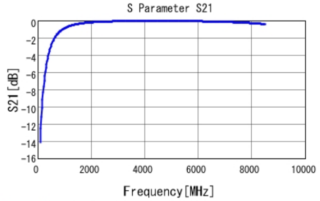
GRM1555C1H3R2CA01 S21 DC0V, 25degC
