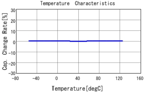
GRM1555C1H3R3BA01 C-Temp. capchange, DC0V, AC1Vrms
