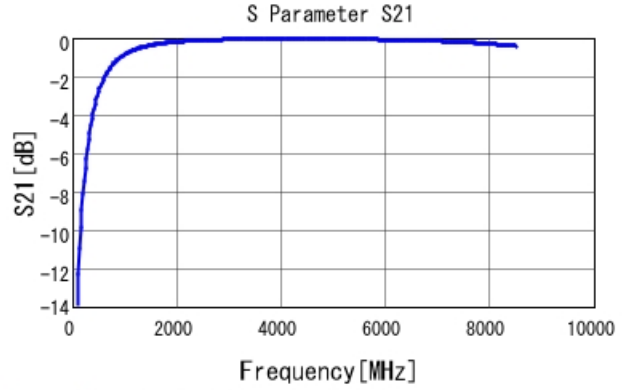
GRM1555C1H3R3BA01 S21 DC0V, 25degC
