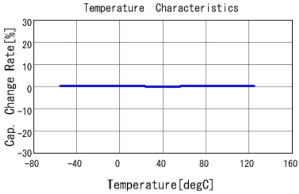
GRM1555C1H3R4BA01 C-Temp. capchange, DC0V, AC1Vrms
