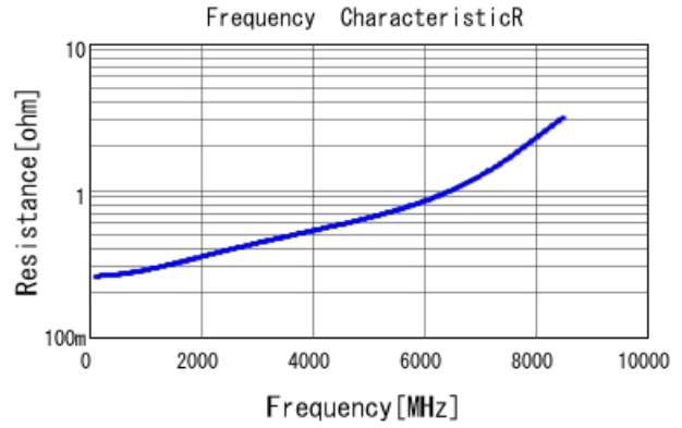
GRM1555C1H3R4BA01 R DCOV, 25degC
