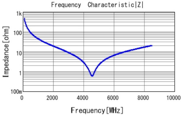
GRM1555C1H3R4BA01 |Z| DCOV, 25degC
