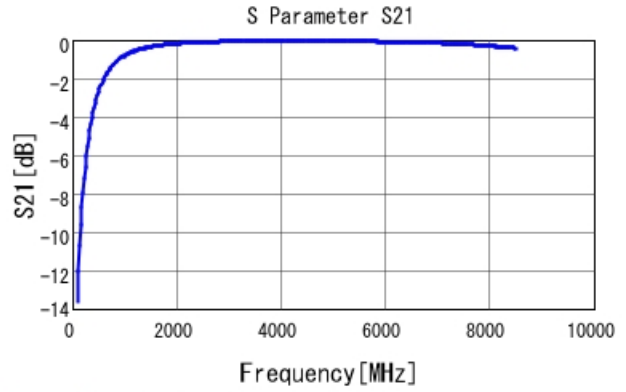
GRM1555C1H3R4BA01 S21 DC0V, 25degC
