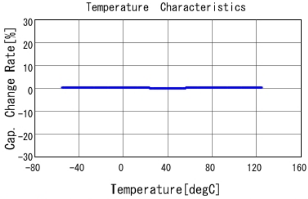
GRM1555C1H3R5BA01 C-Temp. capchange, DC0V, AC1Vrms
