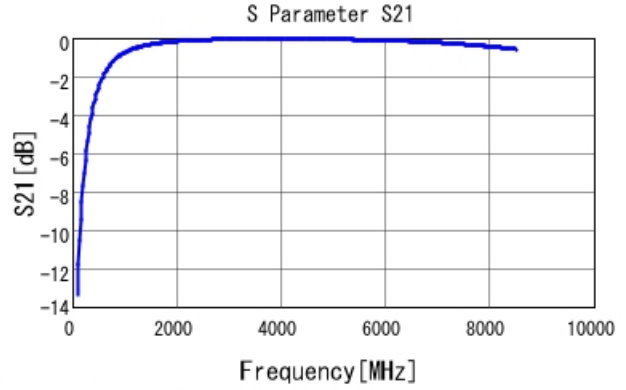
GRM1555C1H3R5BA01 S21 DC0V, 25degC
