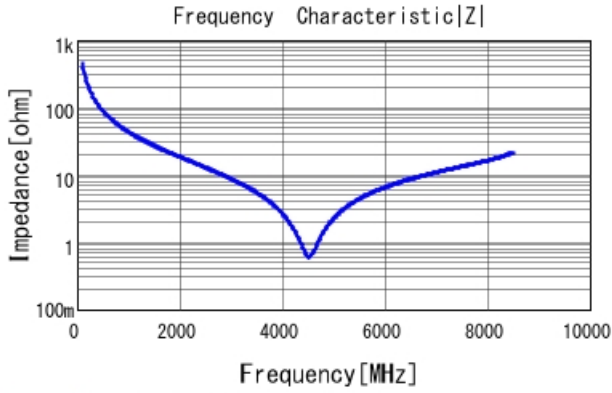
GRM1555C1H3R5BA01 |Z| DCOV, 25degC
