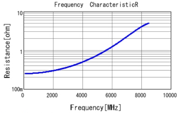
GRM1555C1H3R5BA01 R DCOV, 25degC
