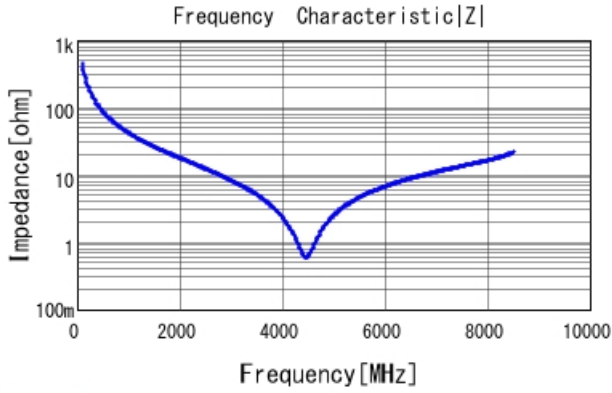
GRM1555C1H3R6BA01 |Z| DCOV, 25degC
