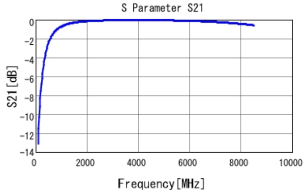
GRM1555C1H3R6BA01 S21 DC0V, 25degC
