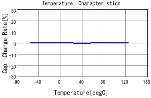
GRM1555C1H3R6CA01 C-Temp. capchange, DCOV, AC1Vrms
