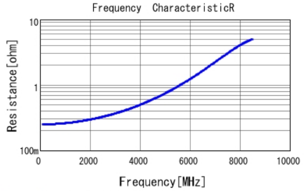
GRM1555C1H3R6CA01 R DCOV, 25degC
