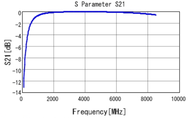
GRM1555C1H3R6CA01 S21 DCOV, 25degC
