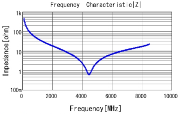
GRM1555C1H3R6CA01 |Z| DCOV, 25degC
