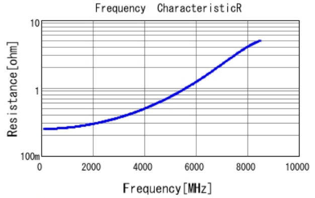
GRM1555C1H3R6WA01 R DCOV, 25degC
