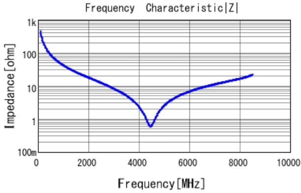
GRM1555C1H3R6WA01 |Z| DCOV, 25degC
