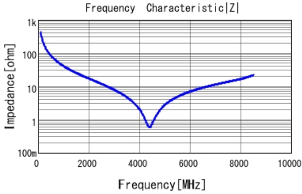
GRM1555C1H3R7BA01 |Z| DCOV, 25degC
