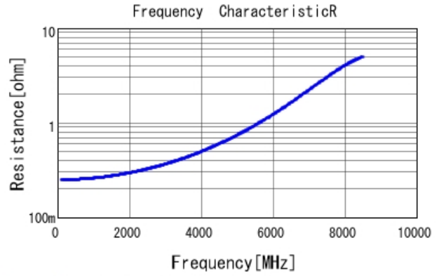
GRM1555C1H3R7BA01 R DCOV, 25degC
