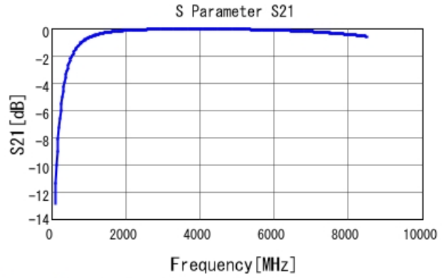
GRM1555C1H3R7BA01 S21 DC0V, 25degC
