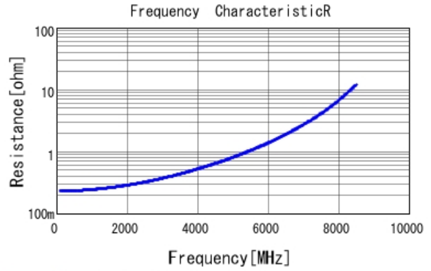
GRM1555C1H3R9BA01 R DCOV, 25degC
