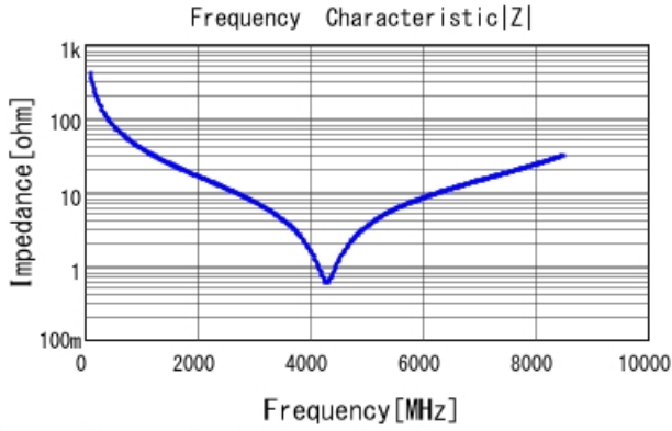
GRM1555C1H3R9BA01 |Z| DCOV, 25degC
