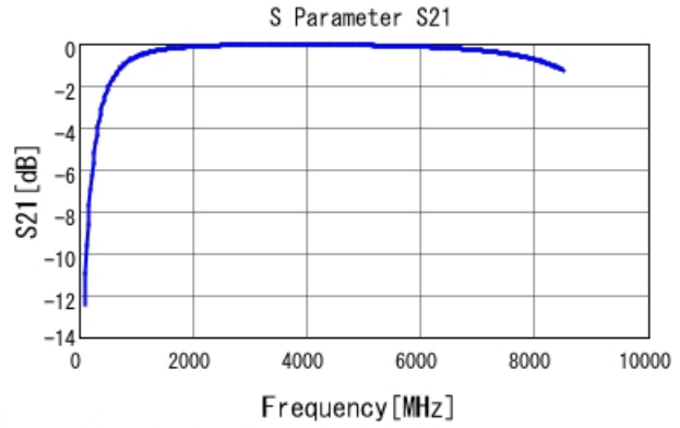
GRM1555C1H3R9BA01 S21 DCOV, 25degC
