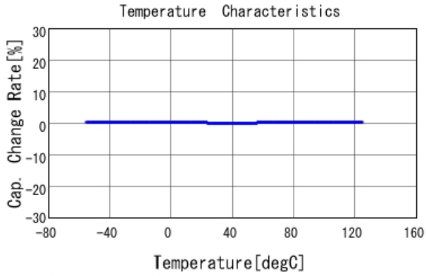
GRM1555C1H3R9BA01 C-Temp. capchange, DCOV, AC1Vrms
