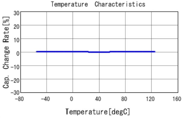
GRM1555C1H3R9CA01 C-Temp. capchange, DCOV, AC1Vrms
