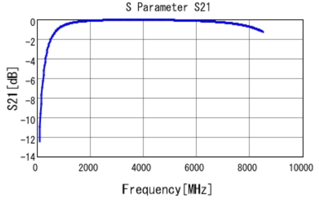
GRM1555C1H3R9CA01 S21 DCOV, 25degC
