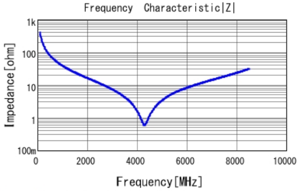
GRM1555C1H3R9CA01 |Z| DCOV, 25degC
