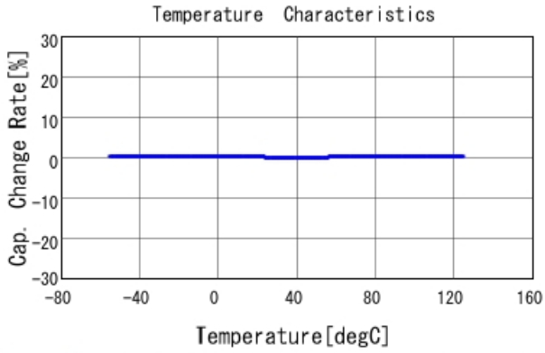
GRM1555C1H3R9WA01 C-Temp. capchange, DCOV, AC1Vrms
