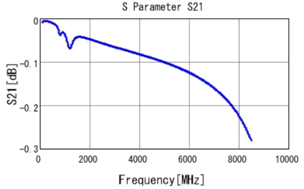
GRM1555C1H471GA01 S21 DCOV, 25degC
