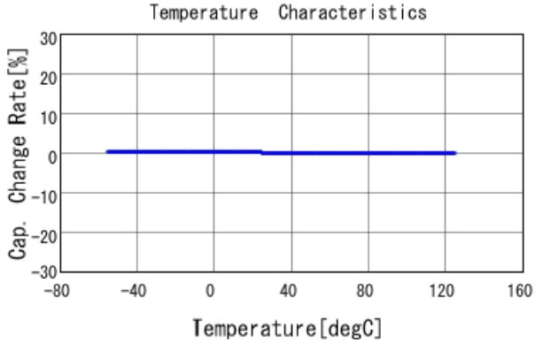
GRM1555C1H471GA01 C-Temp. capchange, DCOV, AC1Vrms
