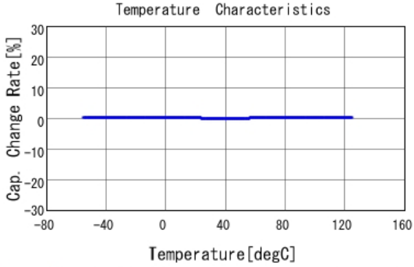
GRM1555C1H4R0CA01 C-Temp. capchange, DCOV, AC1Vrms
