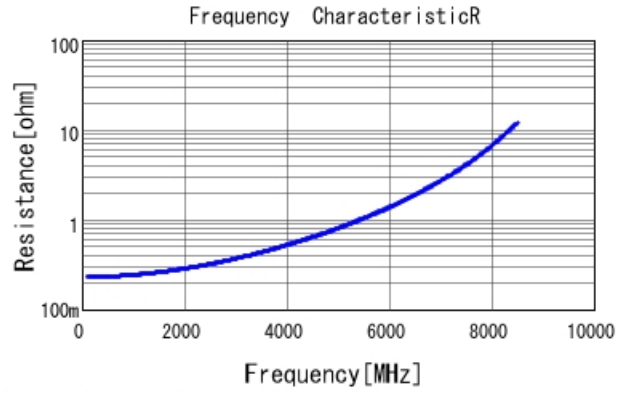
GRM1555C1H4R0CA01 R DCOV, 25degC
