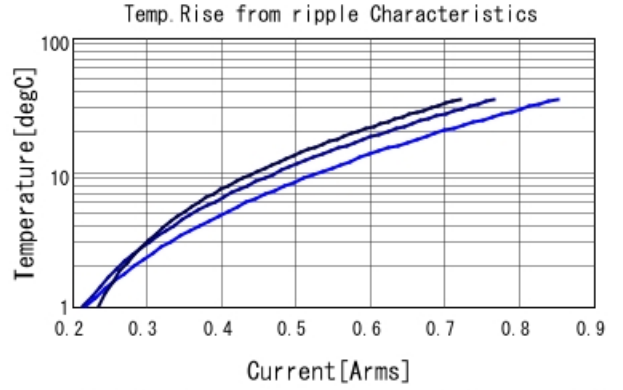
GRM1555C1H4R0CA01 Temp. rise — 1GHz — 2GHz
