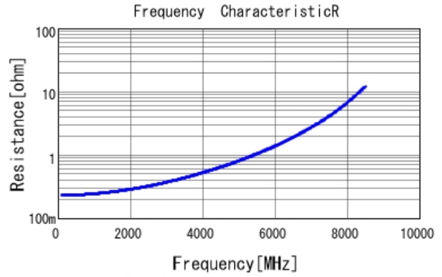
GRM1555C1H4R0WA01 R DCOV, 25degC
