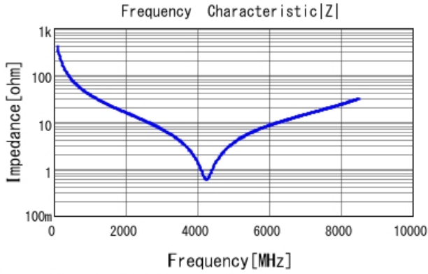
GRM1555C1H4R0WA01 |Z| DCOV, 25degC
