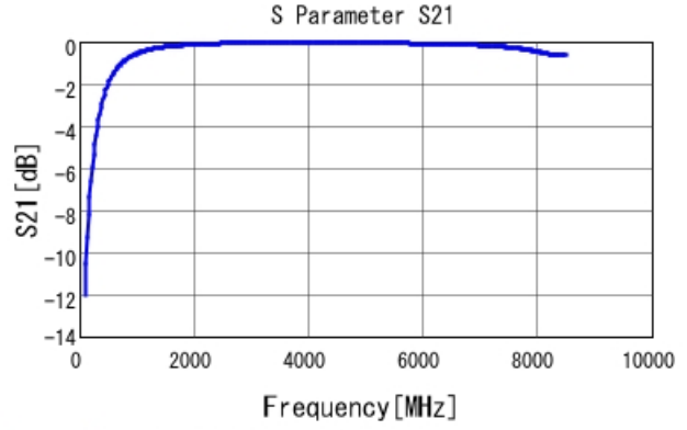
GRM1555C1H4R1BA01 S21 DCOV, 25degC
