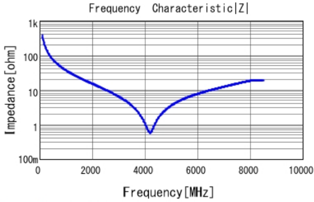
GRM1555C1H4R1BA01 |Z| DCOV, 25degC
