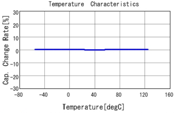
GRM1555C1H4R1BA01 C-Temp. capchange, DCOV, AC1Vrms
