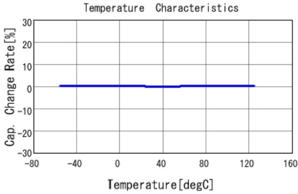
GRM1555C1H4R1CA01 C-Temp. capchange, DCOV, AC1Vrms
