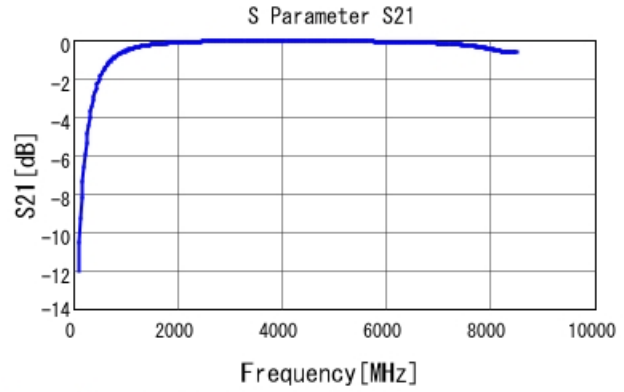
GRM1555C1H4R1CA01 S21 DCOV, 25degC
