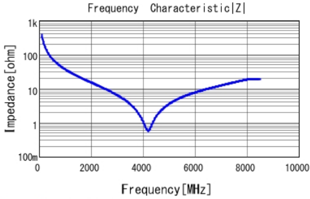
GRM1555C1H4R1CA01 |Z| DCOV, 25degC
