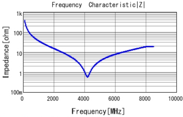
GRM1555C1H4R1WA01 |Z| DCOV, 25degC
