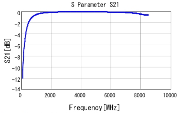
GRM1555C1H4R1WA01 S21 DCOV, 25degC
