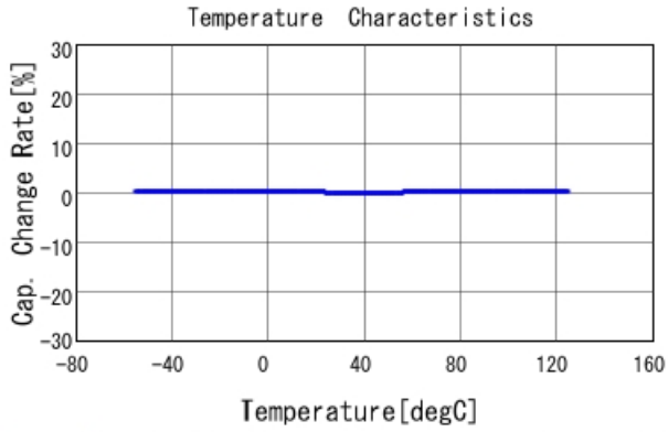
GRM1555C1H4R1WA01 C-Temp. capchange, DCOV, AC1Vrms
