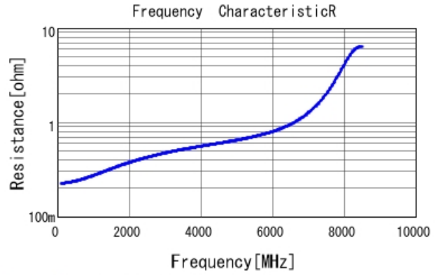
GRM1555C1H4R2BA01 R DCOV, 25degC
