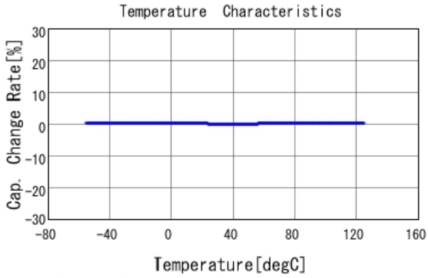
GRM1555C1H4R2BA01 C-Temp. capchange, DC0V, AC1Vrms
