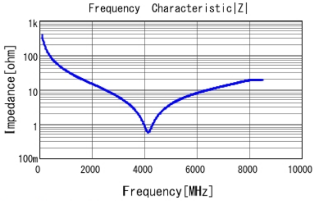
GRM1555C1H4R2BA01 |Z| DCOV, 25degC
