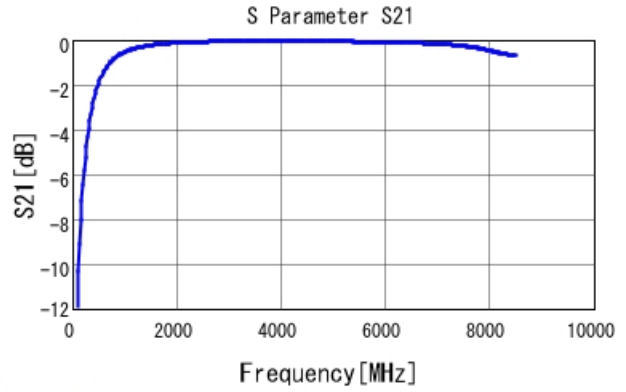
GRM1555C1H4R2BA01 S21 DC0V, 25degC
